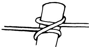
Clove hitch used as an intermediate anchor with tension applied at all times to prevent slipping.
